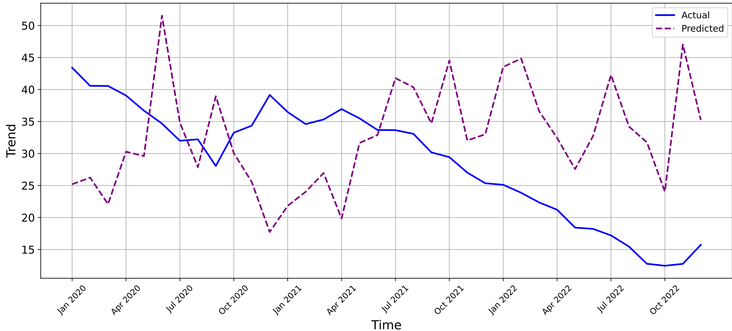
Solution_SSL/TLS_Mentions - Testing
